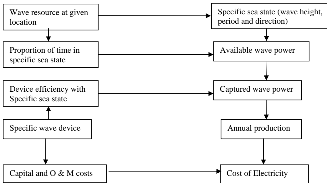
Figure 2: Methodology for appraising WECs [12]
