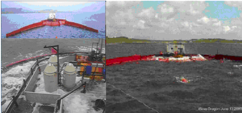
Figure 7: Wave Dragon Overtopping Device [15]
