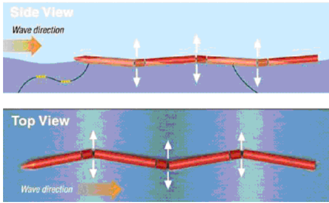
Figure 3: Pelamis [8]
