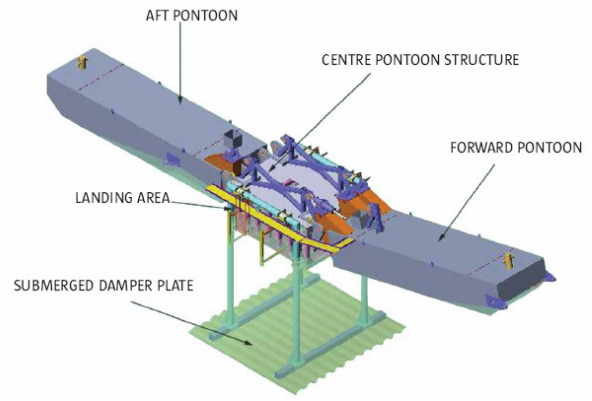
Figure 4: McCabe Wave Pump [8]
