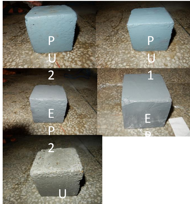
Figure 3: Samples after 120 hours in the acid bath
