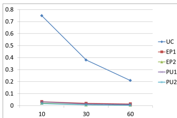
Figure 2: Rate of Absorption against duration omitting the UC Sample
